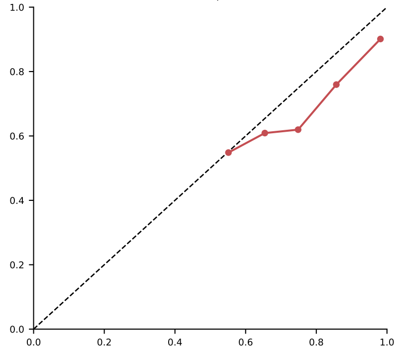
Unusable ECE=0.080, n=2618
